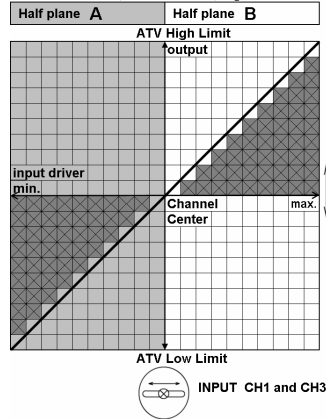
Mix CH3 and CH1, Relation 100%, Sign +
