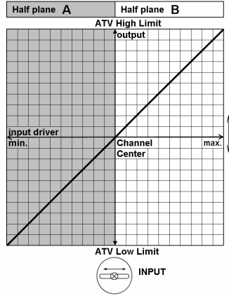
Linear curve, Reverse OFF, Gain 100%
