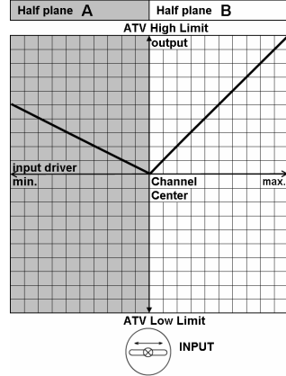
Linear curve, Rev.A ON, Rev.B OFF, Gain A=50%, GB=100%
