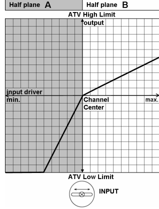
Linear curve, Reverse OFF, Gain A=200%, Gain B=50%
