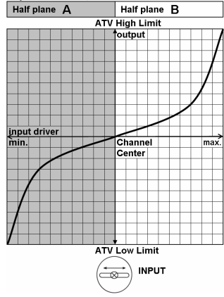
Exponential curve, Reverse OFF Gain 100%
