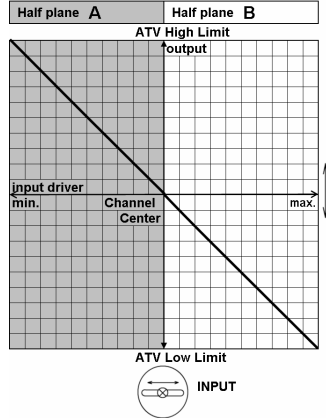
Linear curve, Reverse A and B ON, Gain 100%
