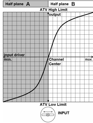
Logarithmical curve, Reverse OFF, Gain 100%
