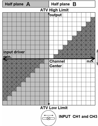
Mix CH1 and CH3, Relation 100%, Sign -
